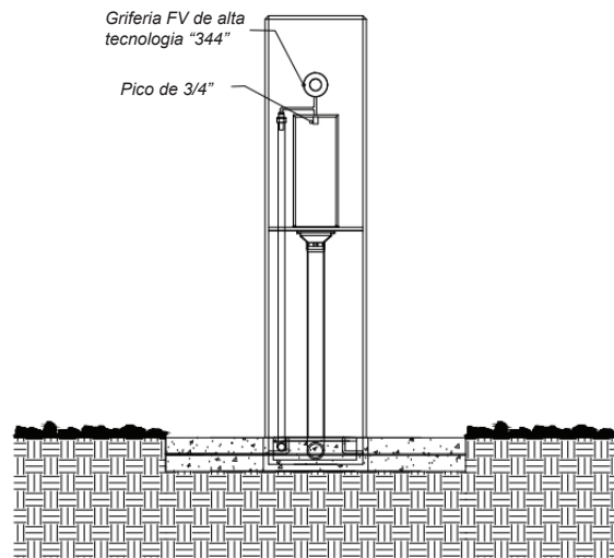
Vista Frontal
