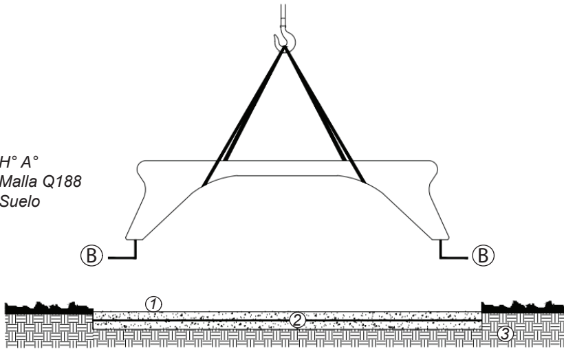
Vista Frontal
